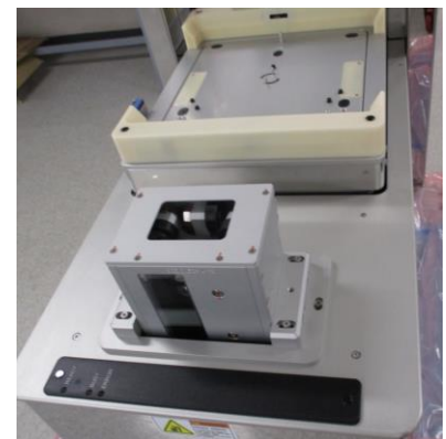
PLM EUV DUAL WITH OHT GUIDE KIT INSTALLED
